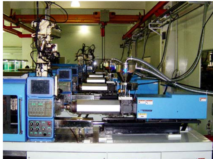
Factory B The conveyance ducts of the system
