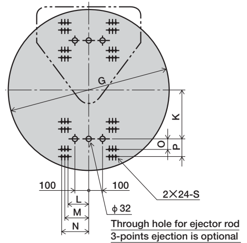
Lower mold side
